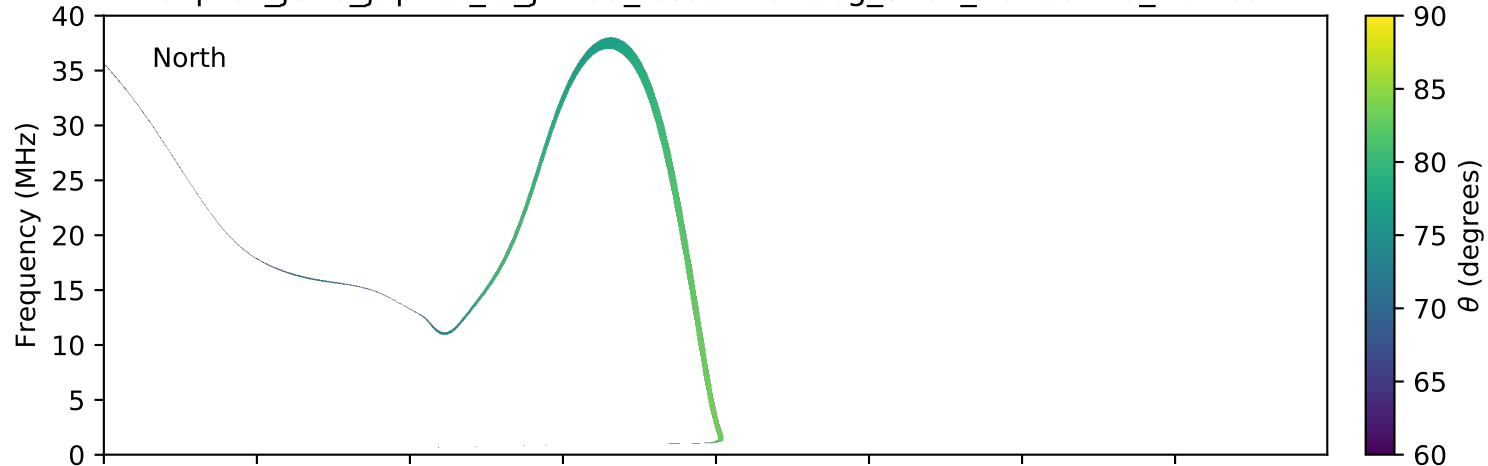
expres_juno_jupiter_io_jrm09_lossc-wid1deg_3kev_20160720_v01.cdf
