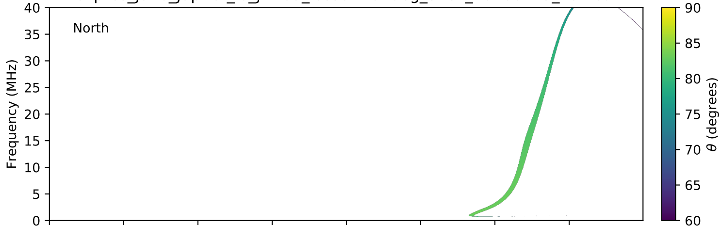
expres_juno_jupiter_io_jrm09_lossc-wid1deg_3kev_20160719_v01.cdf
