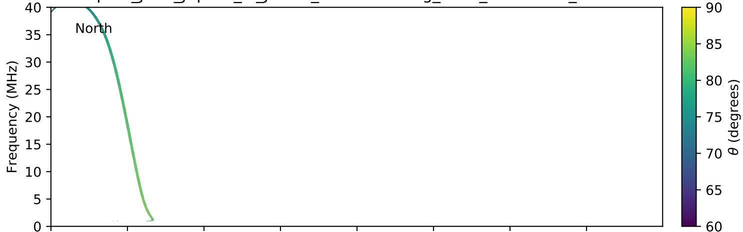
expres_juno_jupiter_io_jrm09_lossc-wid1deg_3kev_20160715_v01.cdf
