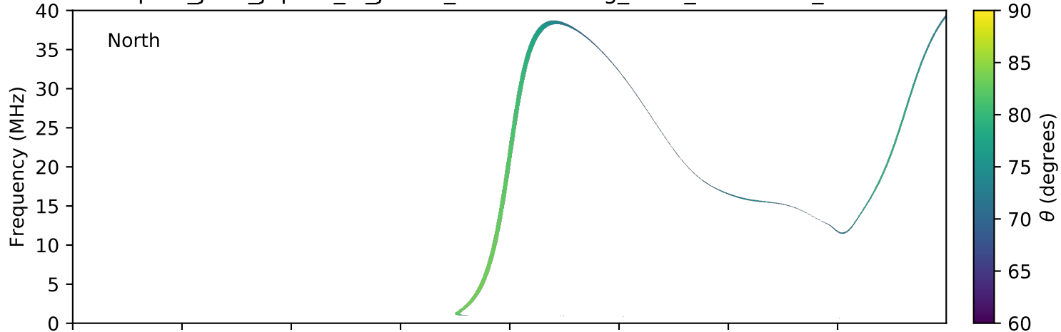
expres_juno_jupiter_io_jrm09_lossc-wid1deg_3kev_20160714_v01.cdf
