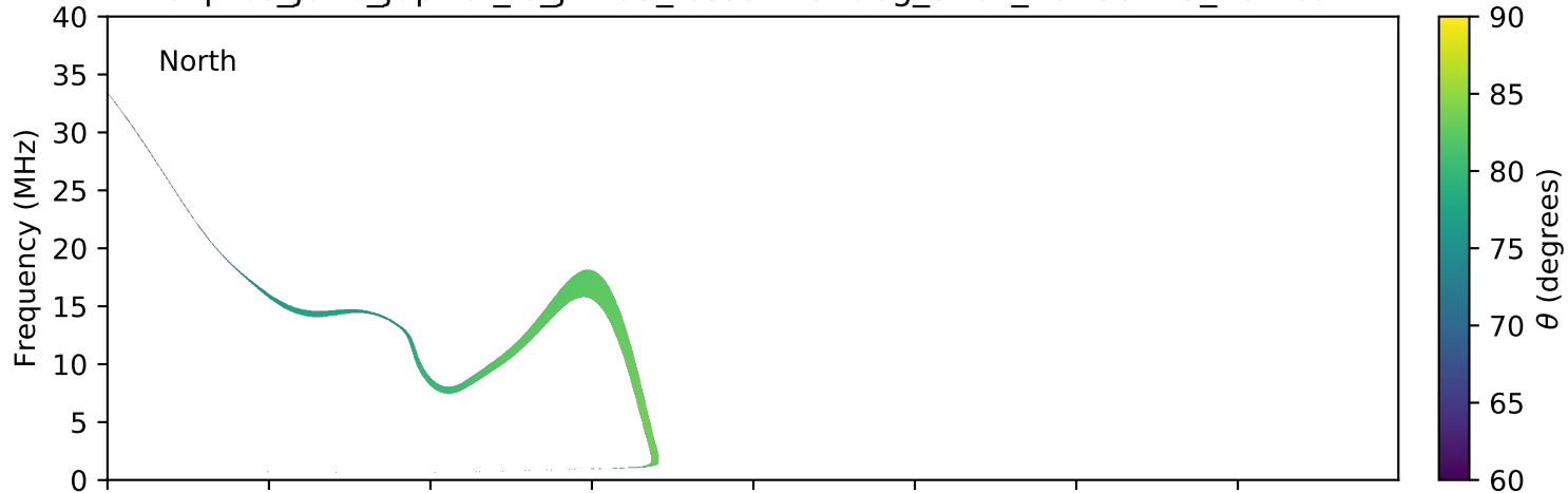
expres_juno_jupiter_io_jrm09_lossc-wid1deg_3kev_20160713_v01.cdf
