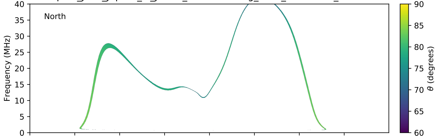
expres_juno_jupiter_io_jrm09_lossc-wid1deg_3kev_20160709_v01.cdf
