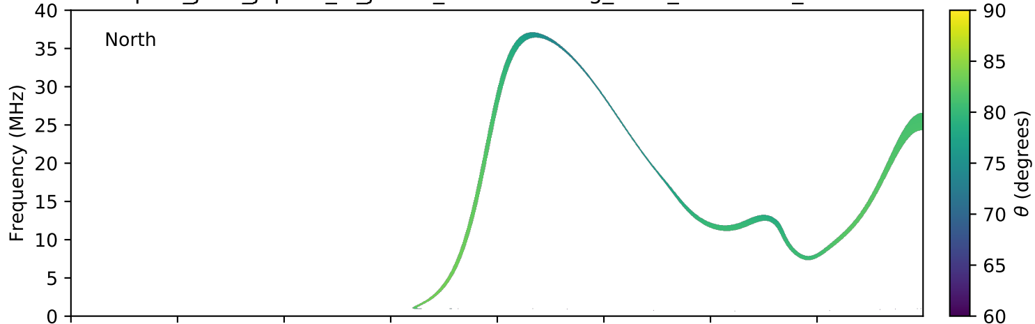
expres_juno_jupiter_io_jrm09_lossc-wid1deg_3kev_20160707_v01.cdf
