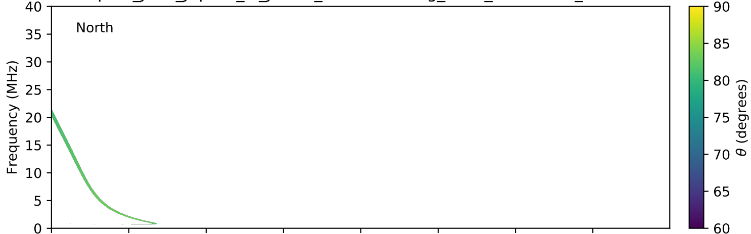
expres_juno_jupiter_io_jrm09_lossc-wid1deg_3kev_20160706_v01.cdf
