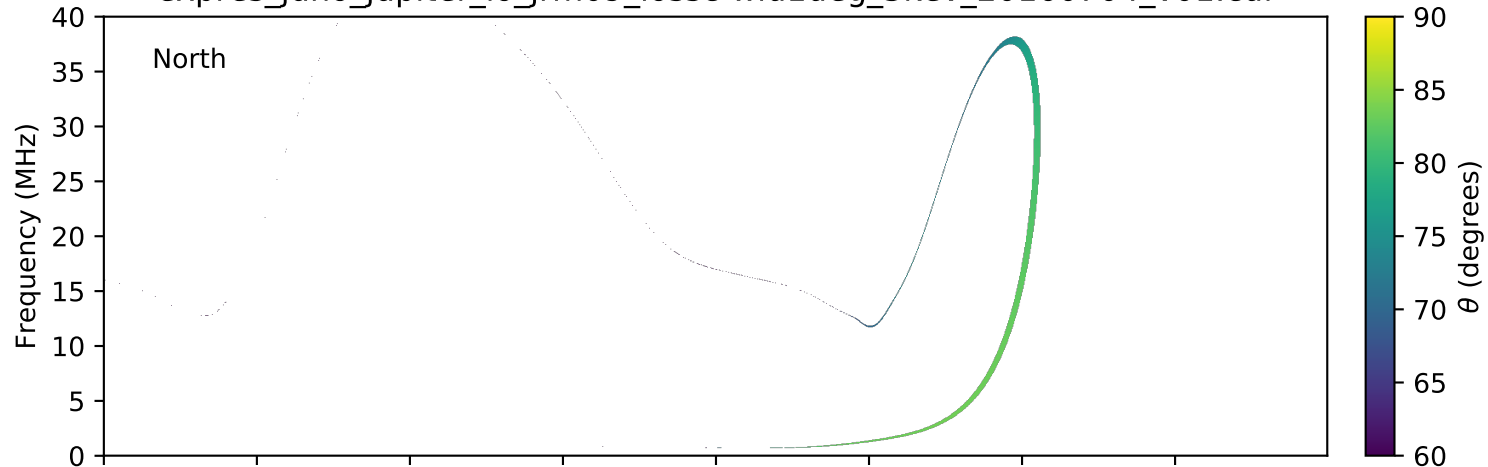
expres_juno_jupiter_io_jrm09_lossc-wid1deg_3kev_20160704_v01.cdf
