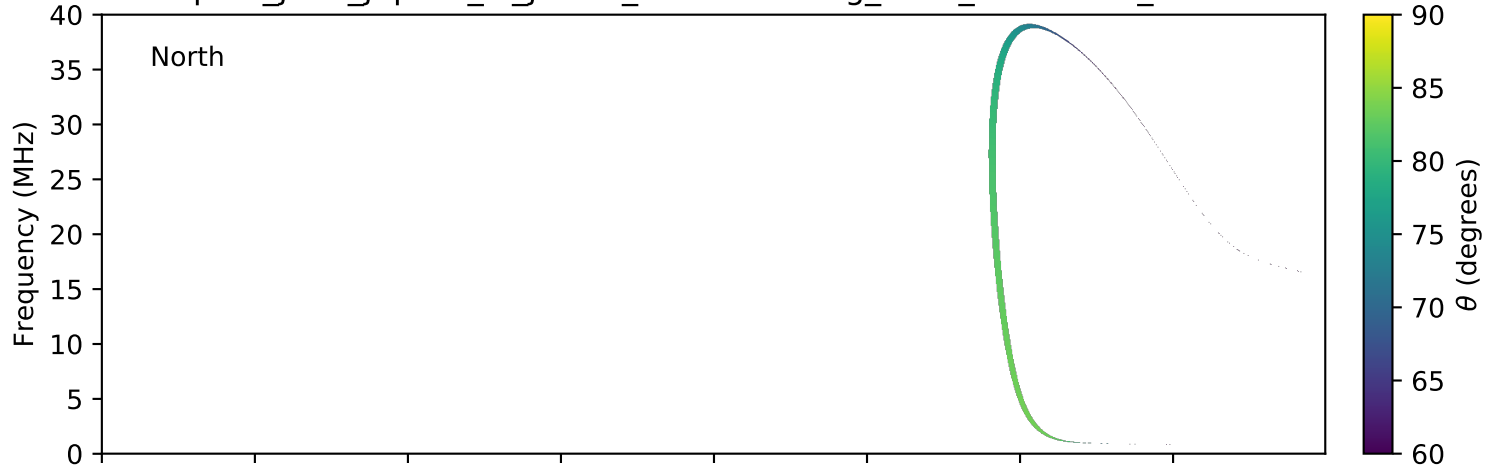
expres_juno_jupiter_io_jrm09_lossc-wid1deg_3kev_20160703_v01.cdf
