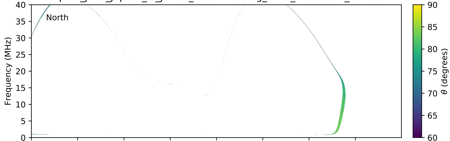
expres_juno_jupiter_io_jrm09_lossc-wid1deg_3kev_20160702_v01.cdf
