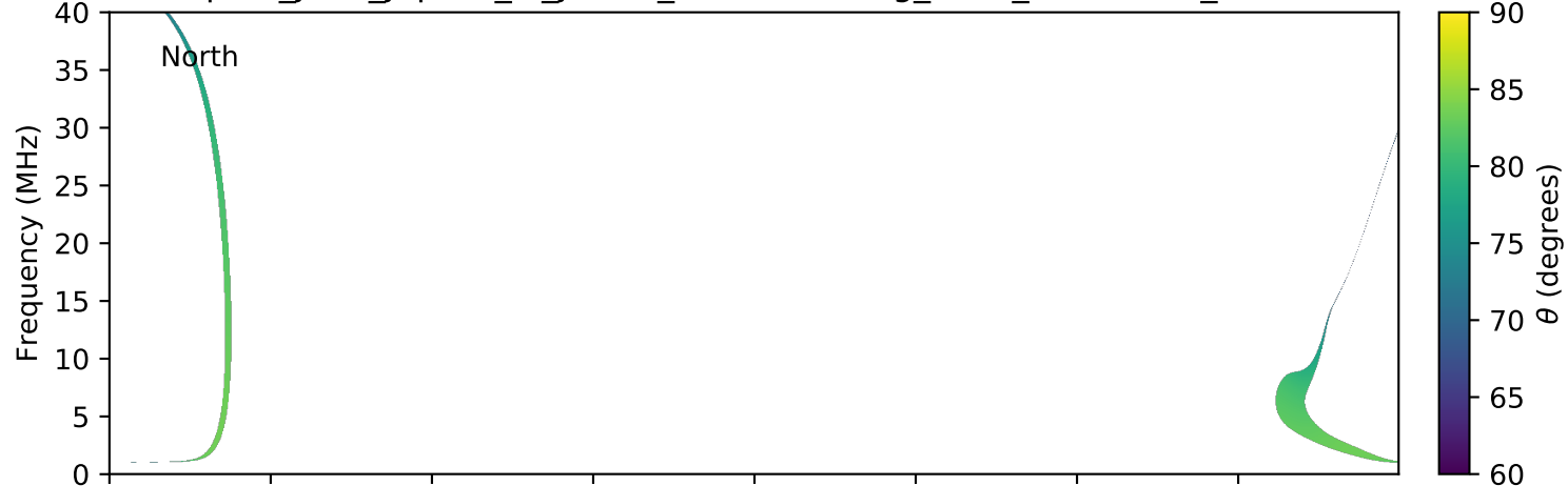
expres_juno_jupiter_io_jrm09_lossc-wid1deg_3kev_20160701_v01.cdf
