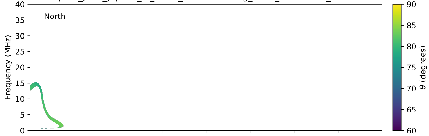
expres_juno_jupiter_io_isaac_lossc-wid1deg_3kev_20160731_v01.cdf
