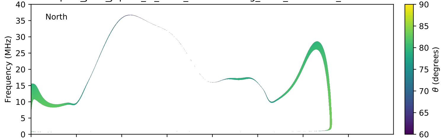
expres_juno_jupiter_io_isaac_lossc-wid1deg_3kev_20160725_v01.cdf
