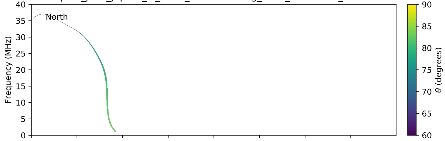
expres_juno_jupiter_io_isaac_lossc-wid1deg_3kev_20160722_v01.cdf
