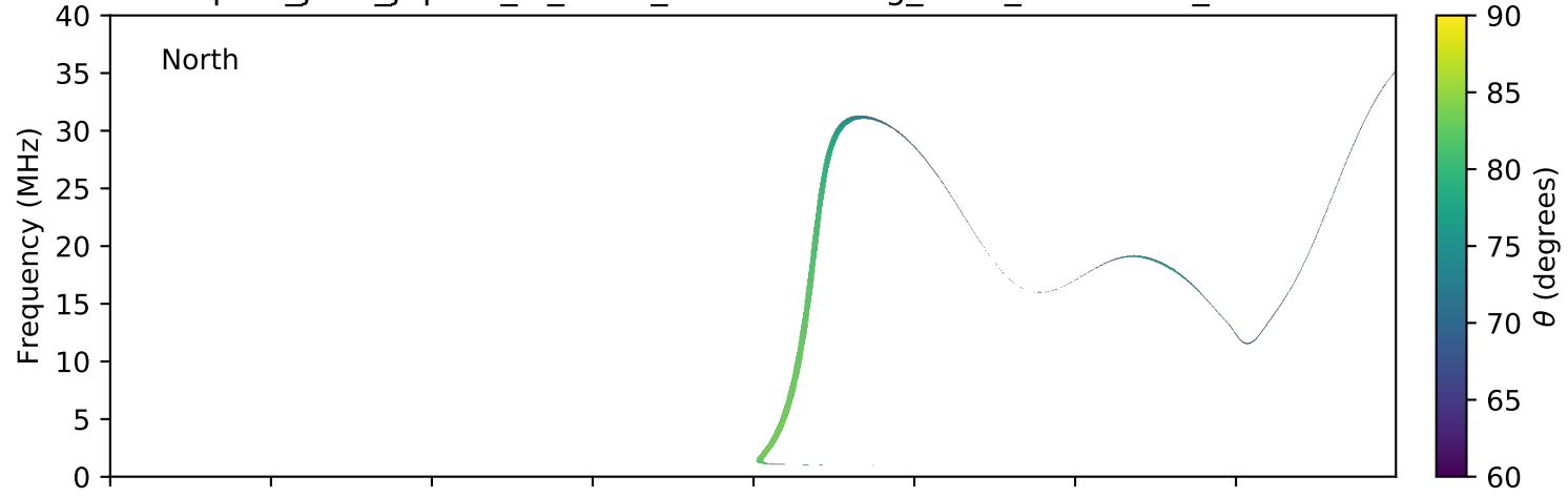
expres_juno_jupiter_io_isaac_lossc-wid1deg_3kev_20160721_v01.cdf
