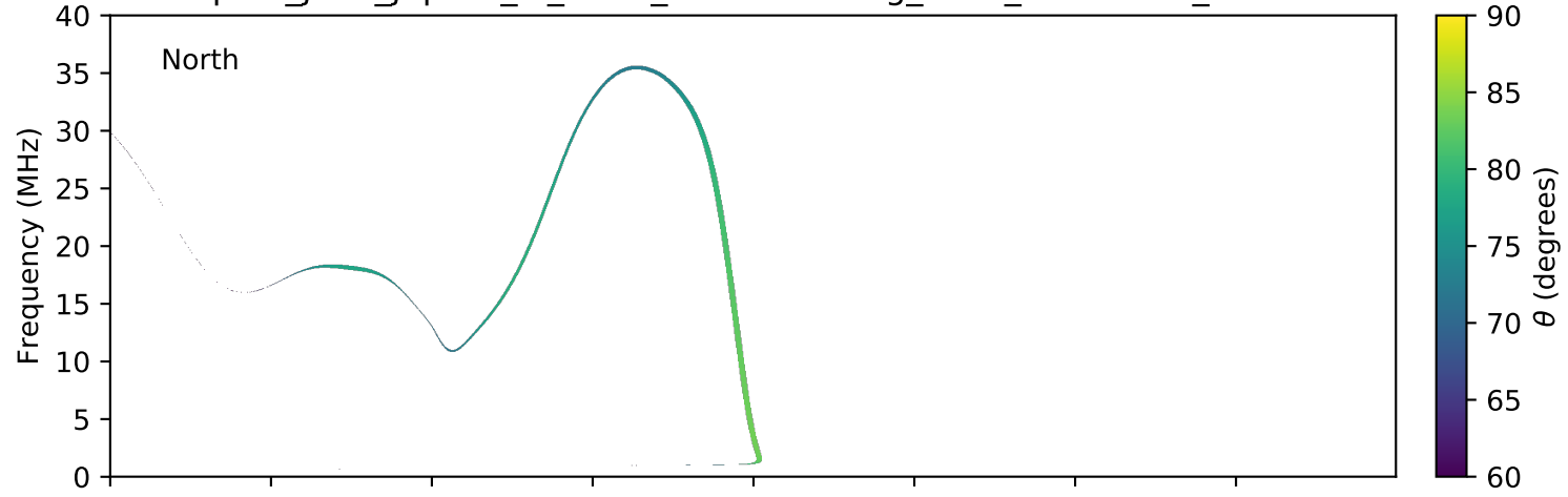
expres_juno_jupiter_io_isaac_lossc-wid1deg_3kev_20160720_v01.cdf
