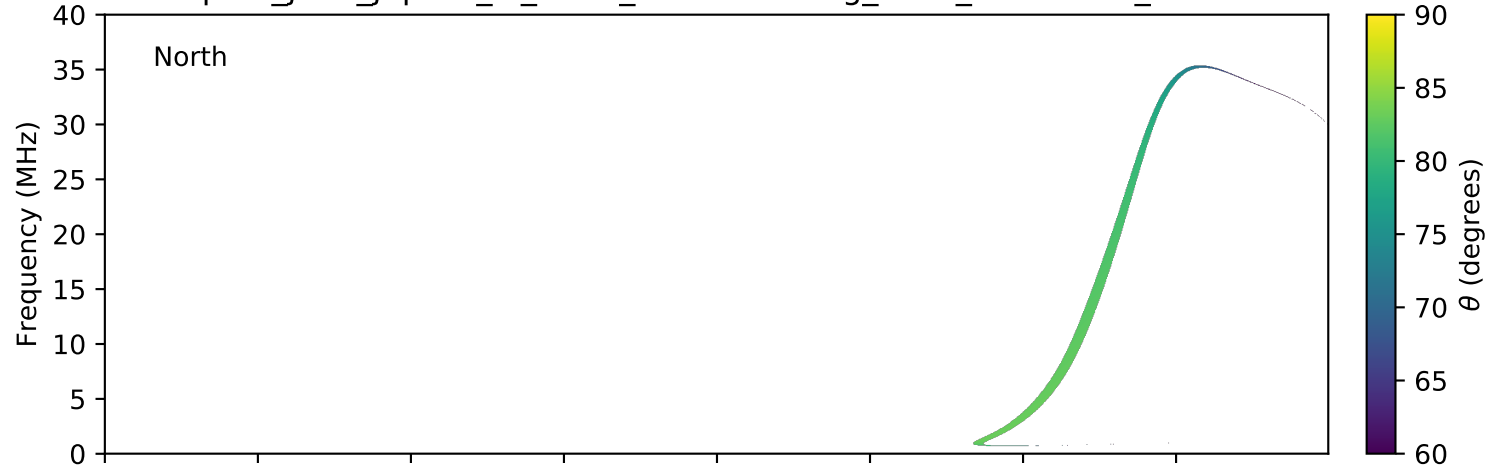
expres_juno_jupiter_io_isaac_lossc-wid1deg_3kev_20160719_v01.cdf
