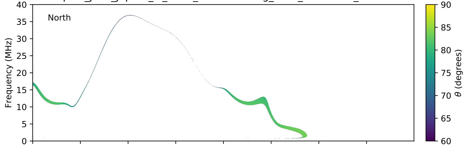
expres_juno_jupiter_io_isaac_lossc-wid1deg_3kev_20160718_v01.cdf
