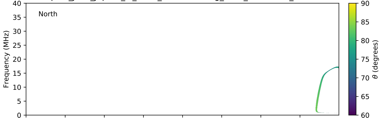
expres_juno_jupiter_io_isaac_lossc-wid1deg_3kev_20160717_v01.cdf
