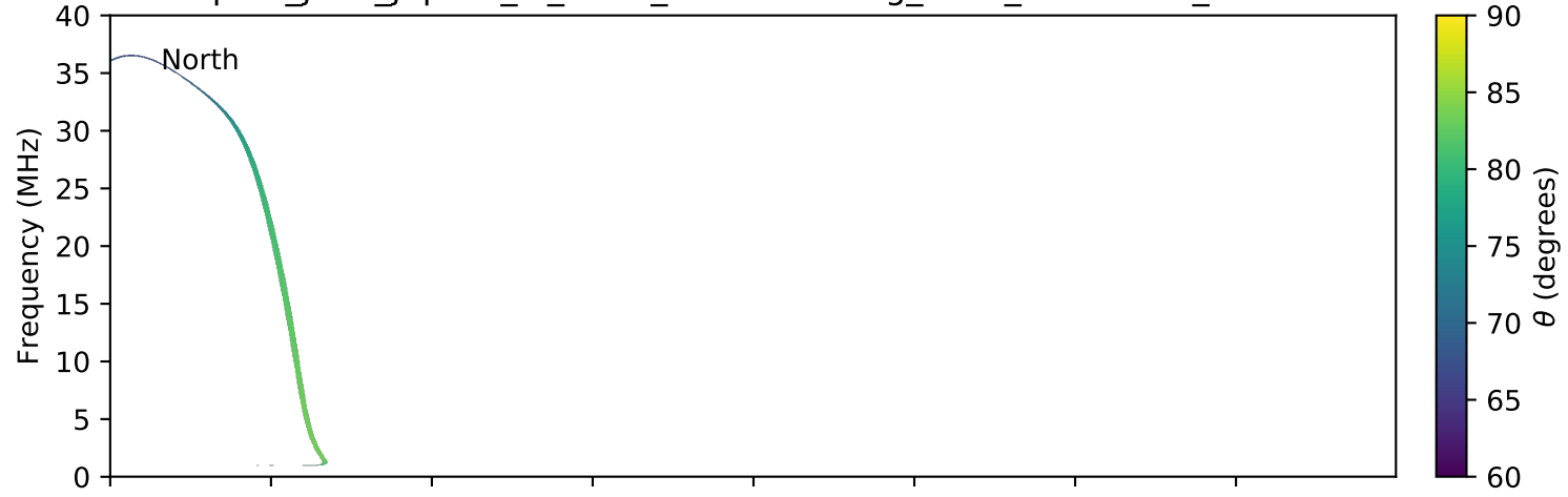
expres_juno_jupiter_io_isaac_lossc-wid1deg_3kev_20160715_v01.cdf
