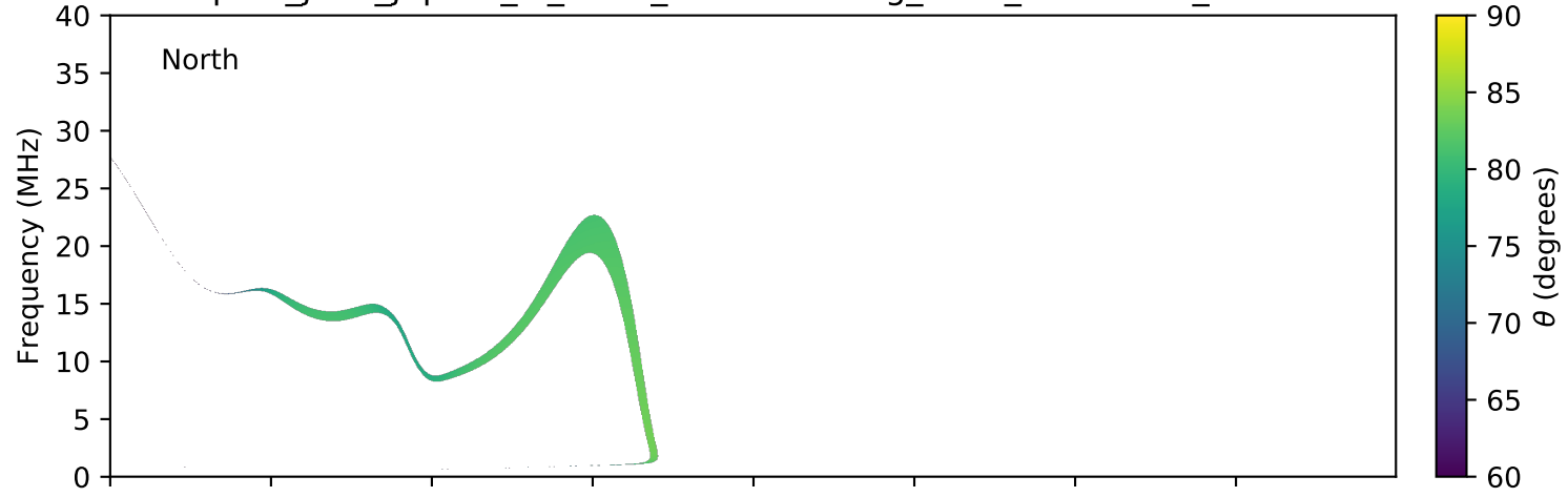
expres_juno_jupiter_io_isaac_lossc-wid1deg_3kev_20160713_v01.cdf
