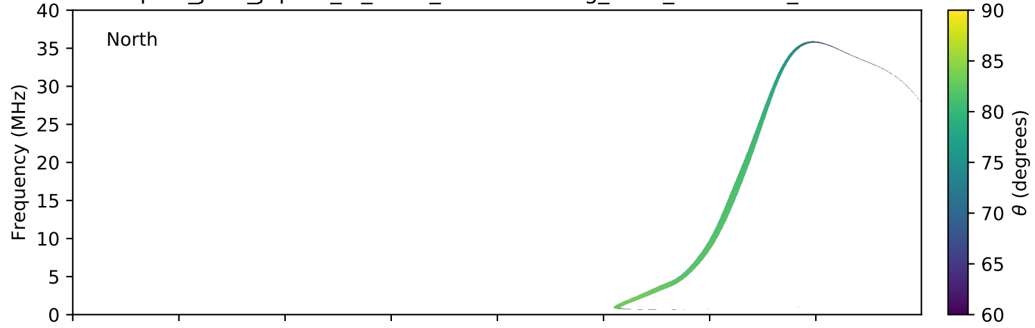
expres_juno_jupiter_io_isaac_lossc-wid1deg_3kev_20160712_v01.cdf
