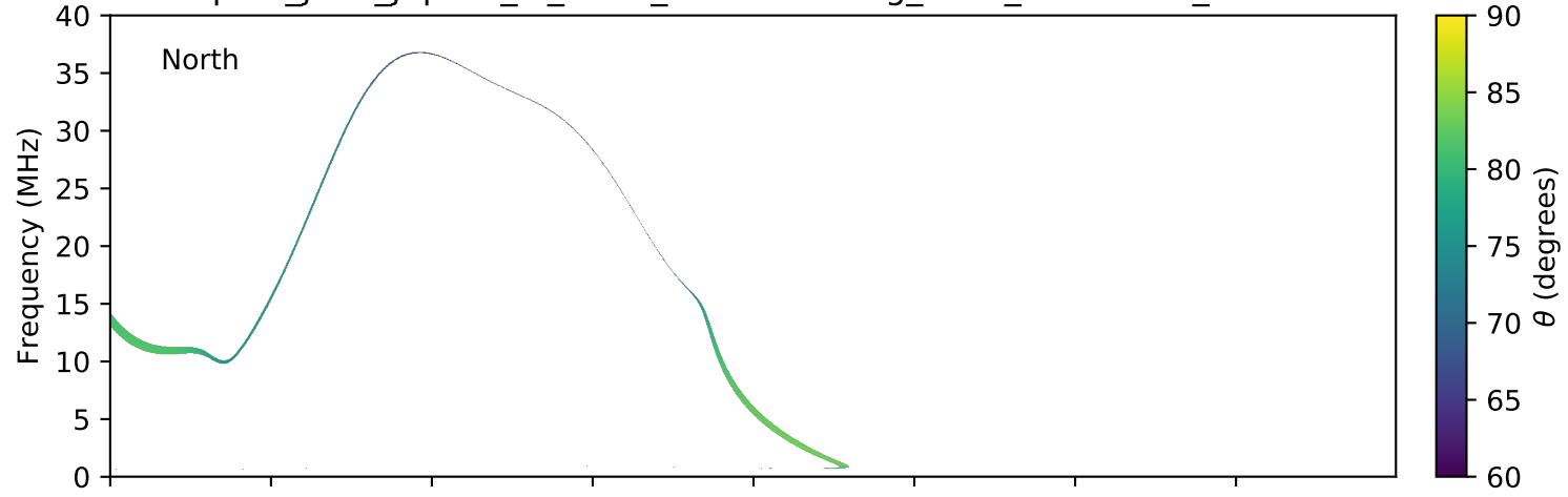
expres_juno_jupiter_io_isaac_lossc-wid1deg_3kev_20160711_v01.cdf
