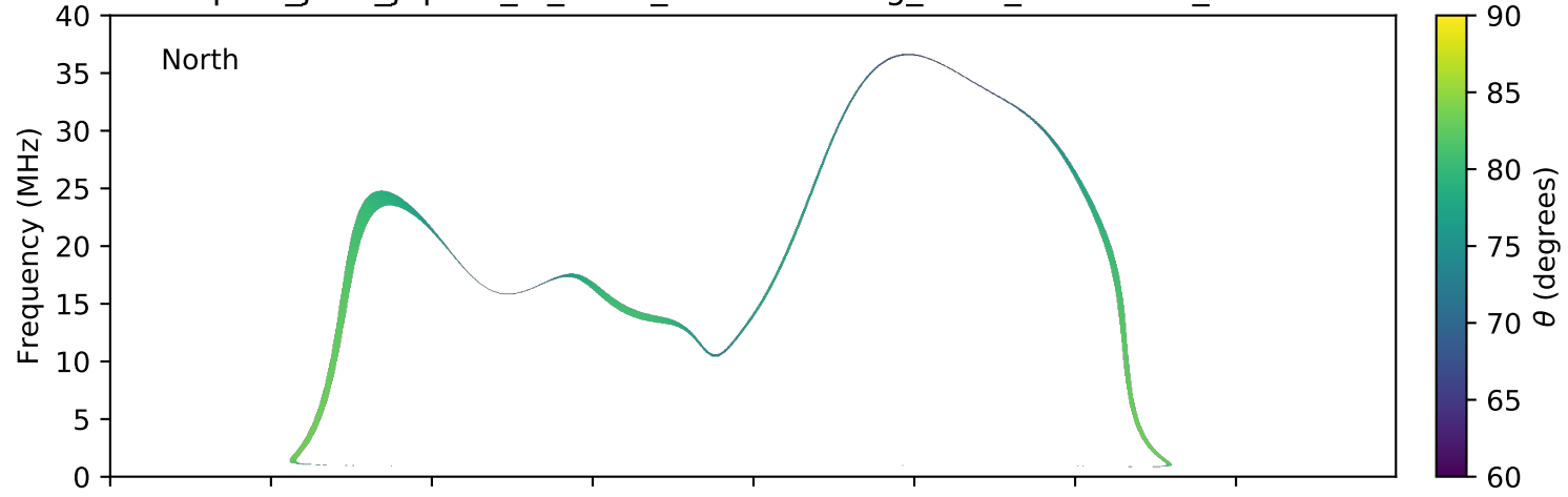
expres_juno_jupiter_io_isaac_lossc-wid1deg_3kev_20160709_v01.cdf
