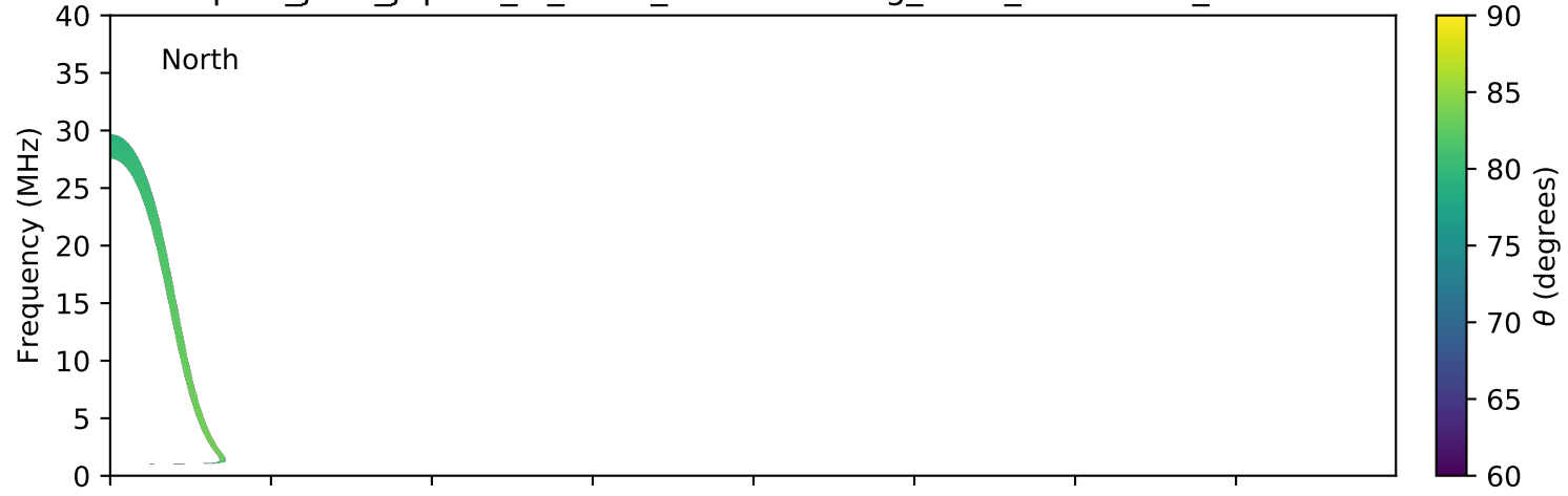
expres_juno_jupiter_io_isaac_lossc-wid1deg_3kev_20160708_v01.cdf
