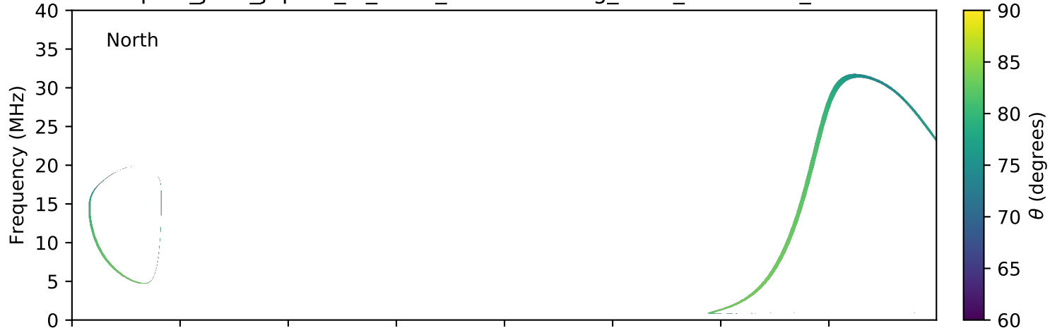
expres_juno_jupiter_io_isaac_lossc-wid1deg_3kev_20160705_v01.cdf
