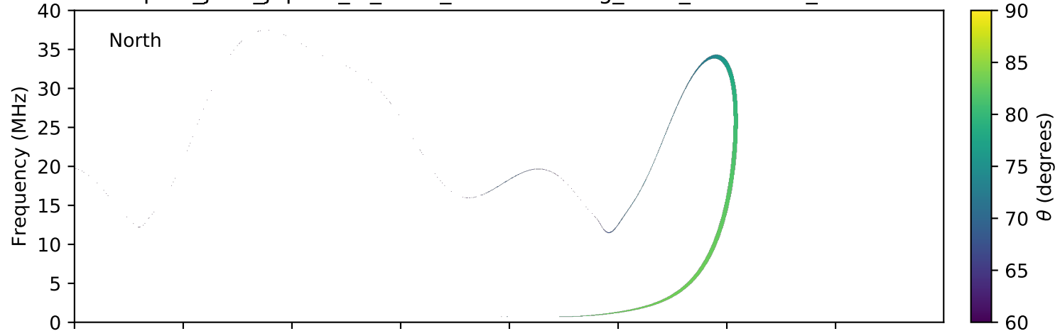
expres_juno_jupiter_io_isaac_lossc-wid1deg_3kev_20160704_v01.cdf
