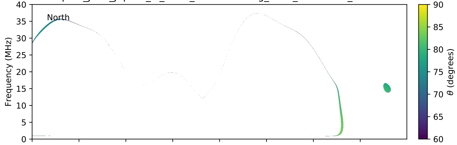
expres_juno_jupiter_io_isaac_lossc-wid1deg_3kev_20160702_v01.cdf
