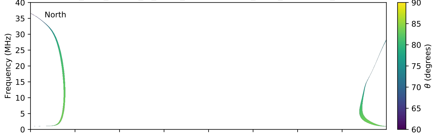
expres_juno_jupiter_io_isaac_lossc-wid1deg_3kev_20160701_v01.cdf
