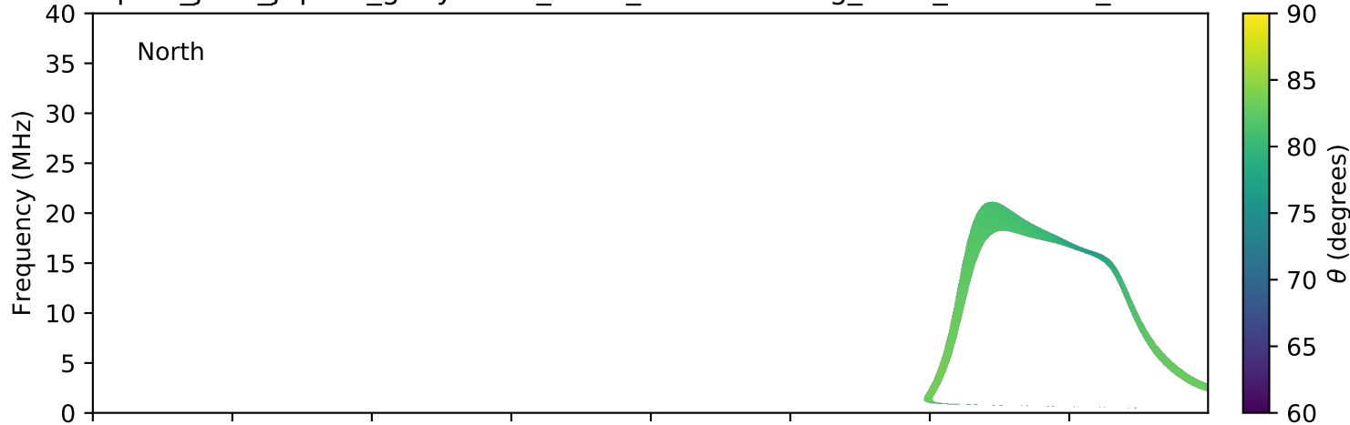
expres_juno_jupiter_ganymede_isaac_lossc-wid1deg_3kev_20160727_v01.cdf
