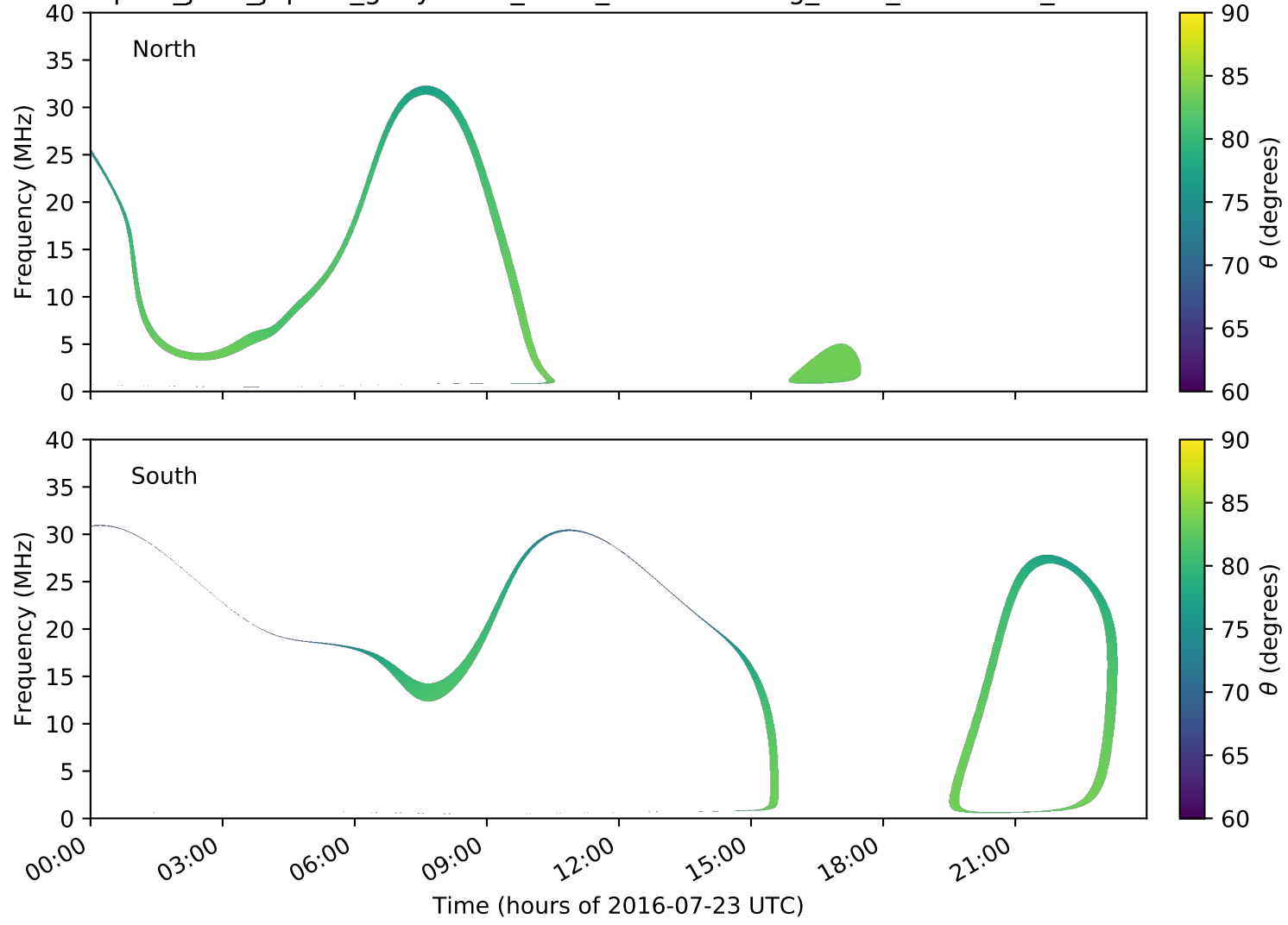
expres_juno_jupiter_ganymede_isaac_lossc-wid1deg_3kev_20160723_v01.cdf
