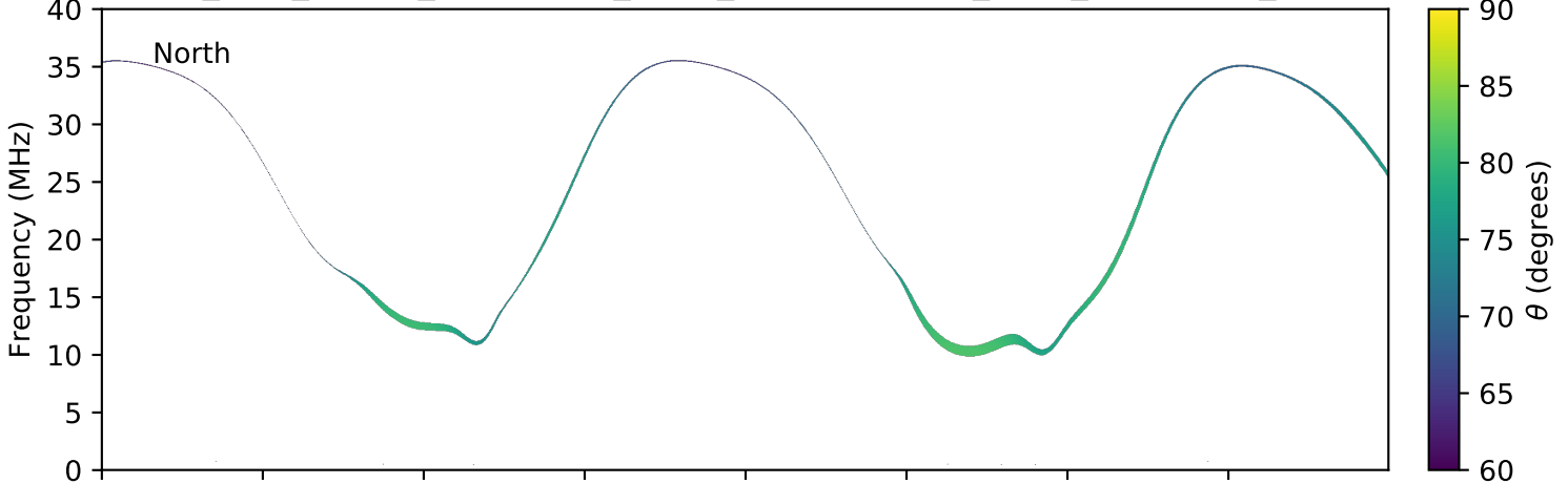
expres_juno_jupiter_ganymede_isaac_lossc-wid1deg_3kev_20160722_v01.cdf
