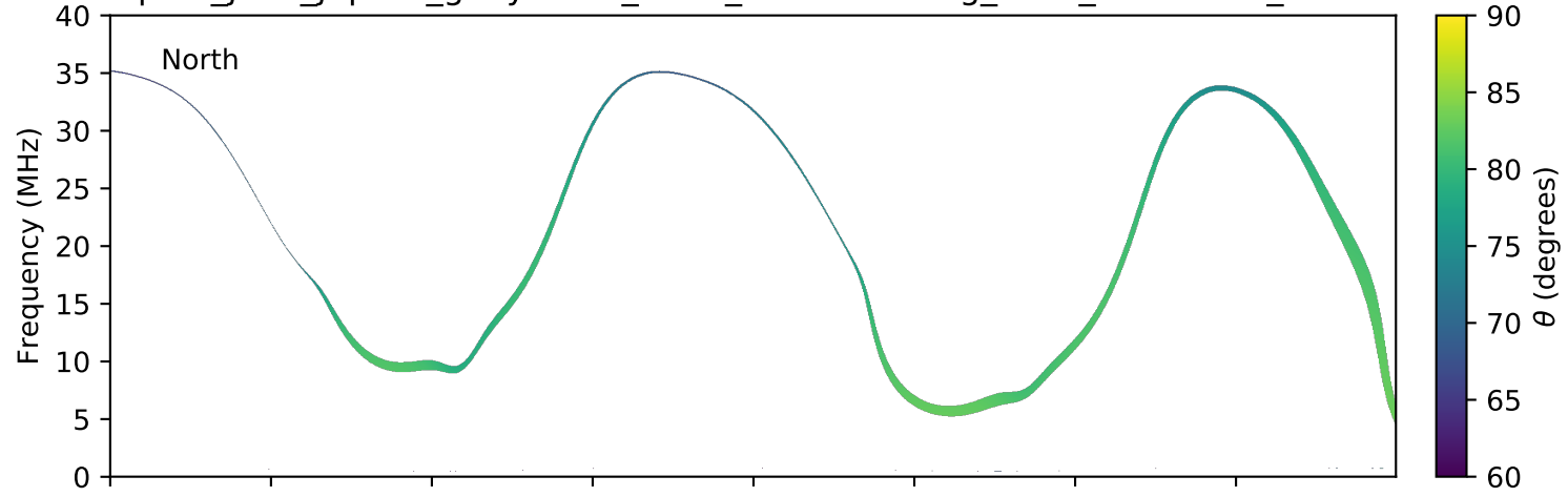
expres_juno_jupiter_ganymede_isaac_lossc-wid1deg_3kev_20160715_v01.cdf
