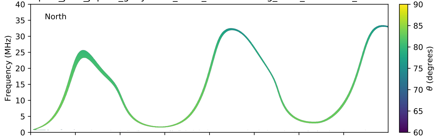
expres_juno_jupiter_ganymede_isaac_lossc-wid1deg_3kev_20160707_v01.cdf
