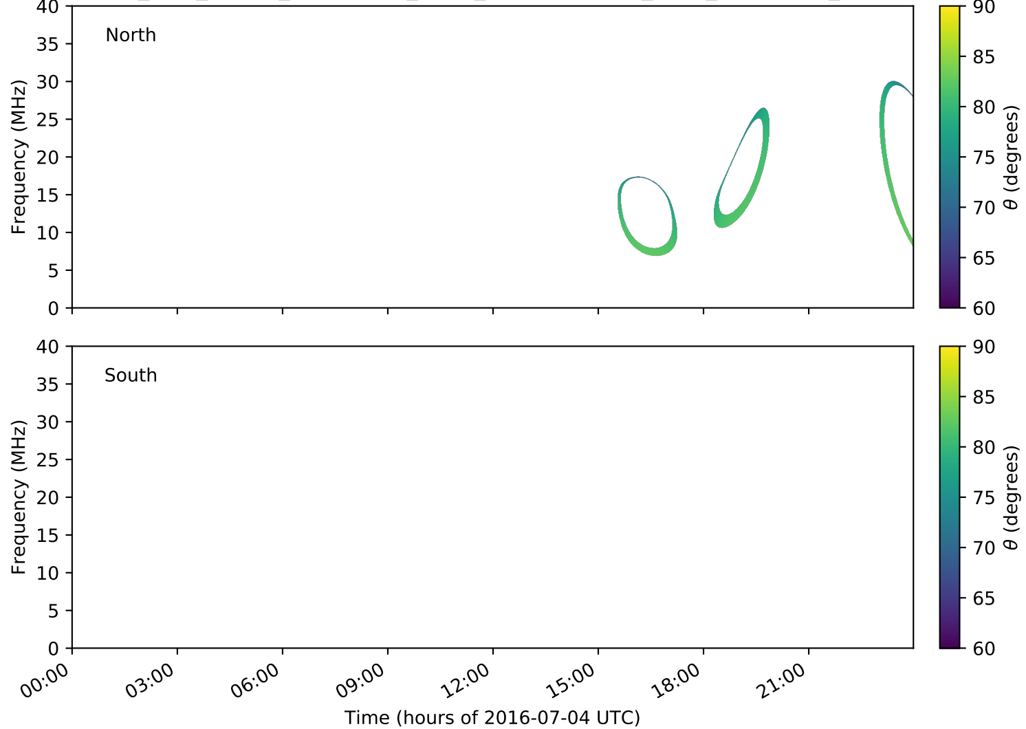
expres_juno_jupiter_ganymede_isaac_lossc-wid1deg_3kev_20160704_v01.cdf
