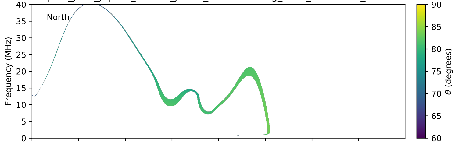
expres_juno_jupiter_europa_jrm09_lossc-wid1deg_3kev_20160731_v01.cdf
