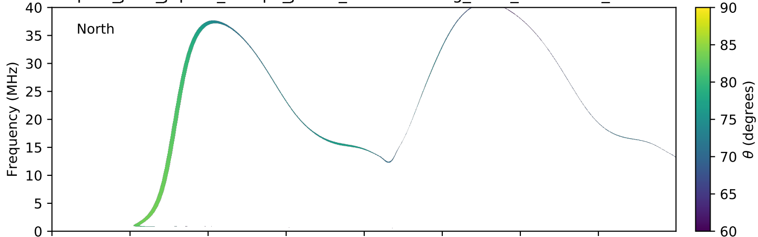
expres_juno_jupiter_europa_jrm09_lossc-wid1deg_3kev_20160730_v01.cdf
