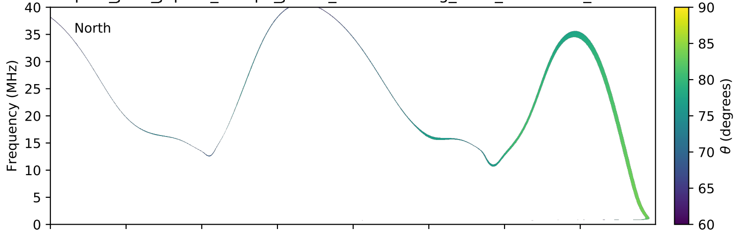
expres_juno_jupiter_europa_jrm09_lossc-wid1deg_3kev_20160727_v01.cdf
