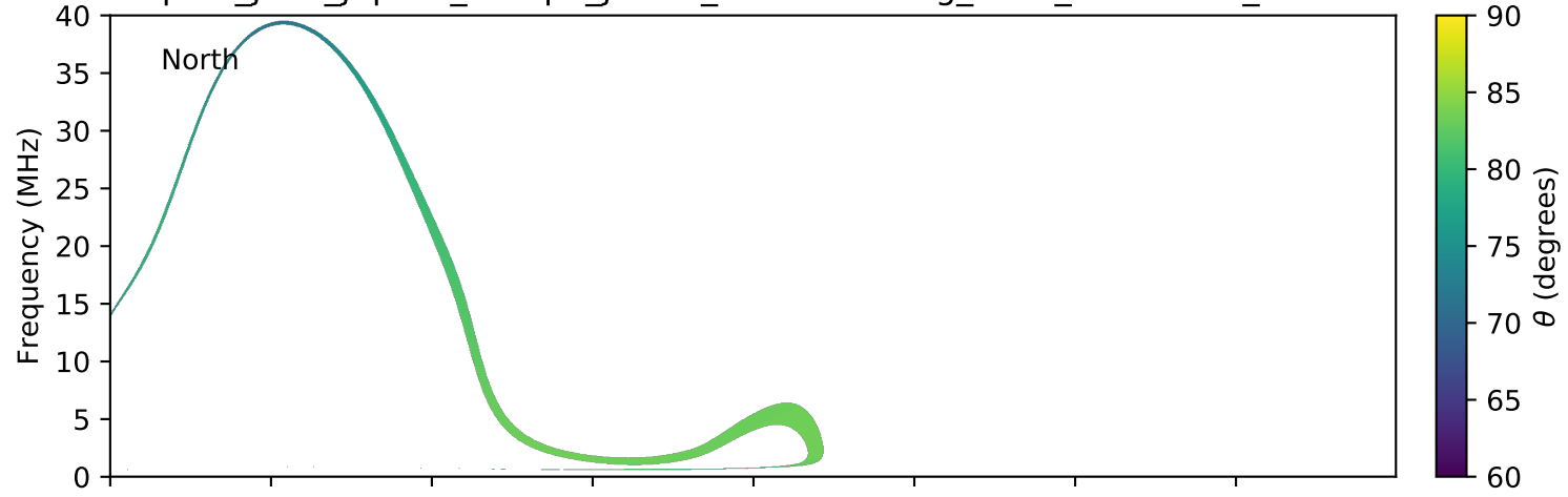
expres_juno_jupiter_europa_jrm09_lossc-wid1deg_3kev_20160724_v01.cdf
