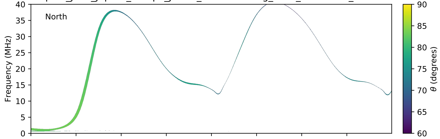
expres_juno_jupiter_europa_jrm09_lossc-wid1deg_3kev_20160723_v01.cdf
