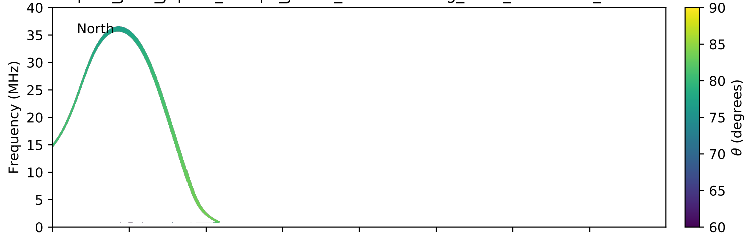
expres_juno_jupiter_europa_jrm09_lossc-wid1deg_3kev_20160717_v01.cdf
