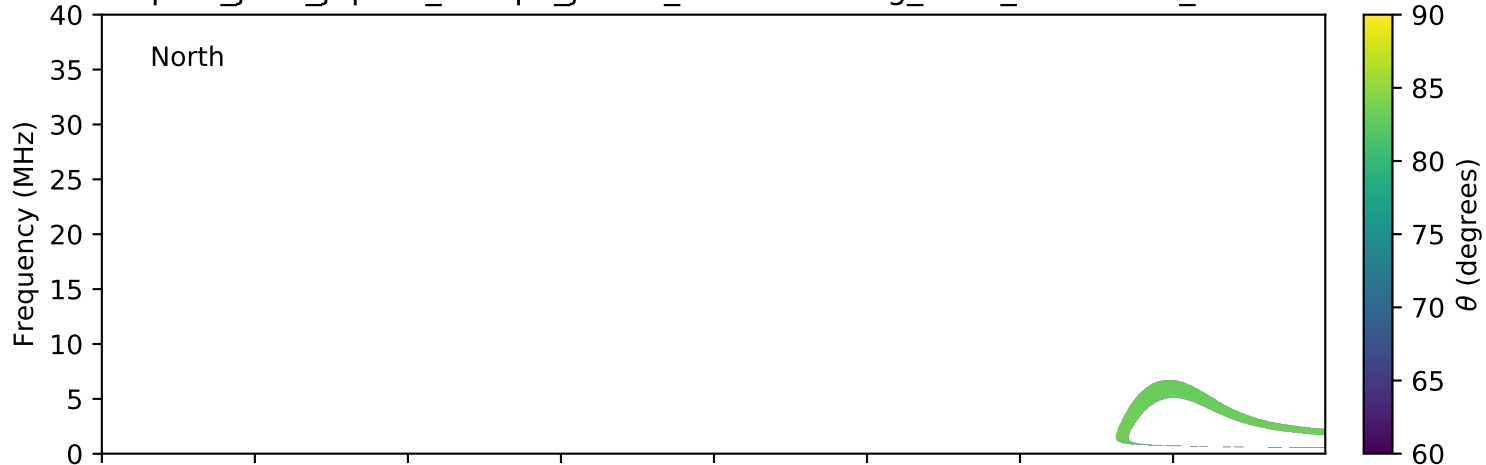
expres_juno_jupiter_europa_jrm09_lossc-wid1deg_3kev_20160715_v01.cdf
