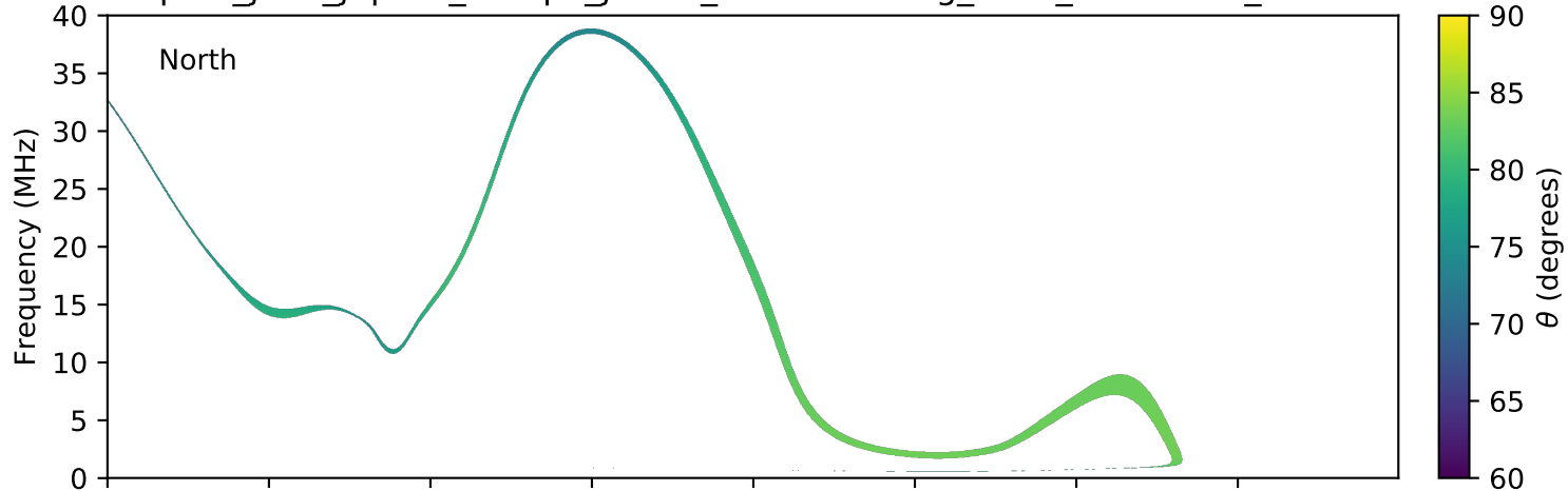
expres_juno_jupiter_europa_jrm09_lossc-wid1deg_3kev_20160713_v01.cdf
