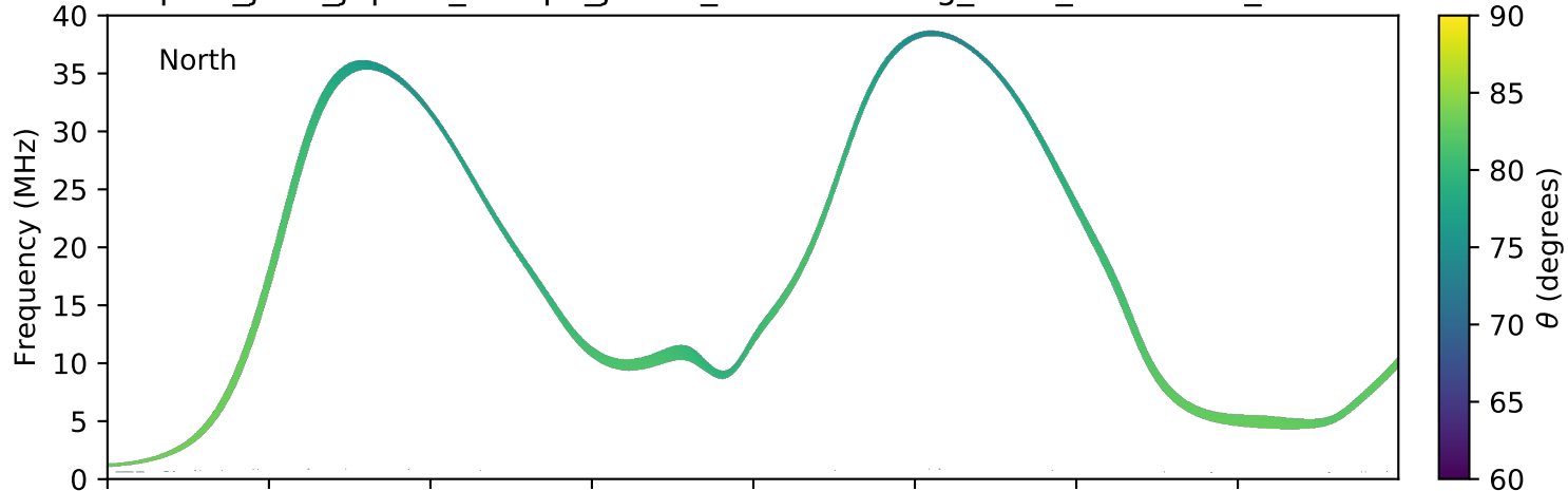
expres_juno_jupiter_europa_jrm09_lossc-wid1deg_3kev_20160709_v01.cdf
