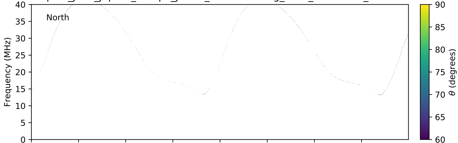
expres_juno_jupiter_europa_jrm09_lossc-wid1deg_3kev_20160702_v01.cdf
