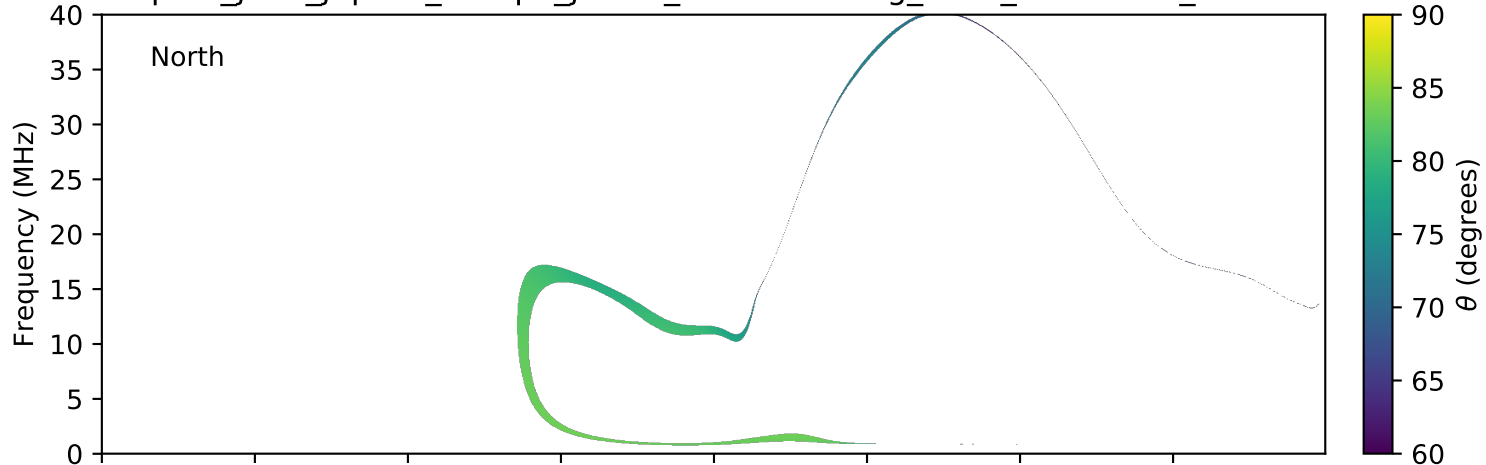
expres_juno_jupiter_europa_jrm09_lossc-wid1deg_3kev_20160701_v01.cdf
