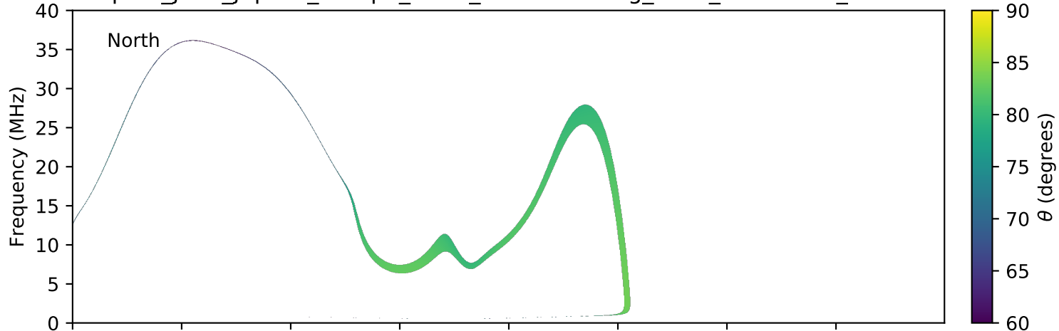
expres_juno_jupiter_europa_isaac_lossc-wid1deg_3kev_20160731_v01.cdf
