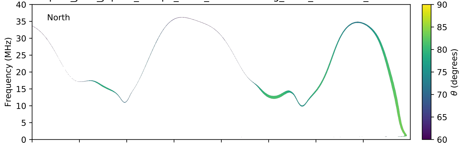
expres_juno_jupiter_europa_isaac_lossc-wid1deg_3kev_20160727_v01.cdf
