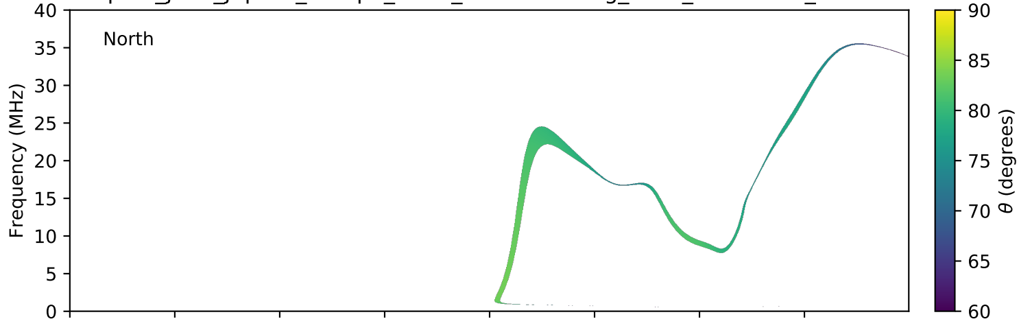
expres_juno_jupiter_europa_isaac_lossc-wid1deg_3kev_20160726_v01.cdf
